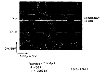
Fig. 33 - Envelope-detector-circuit waveforms.
