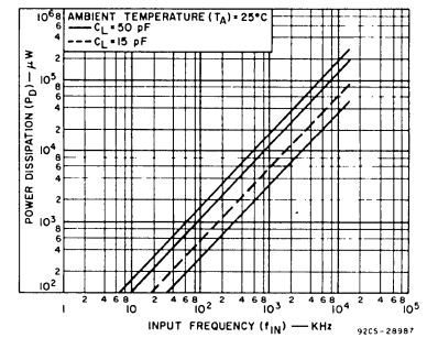
Fig. 13 - Dynamic power dissipation.
