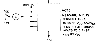
Fig. 9 - Input leakage current test circuit.
