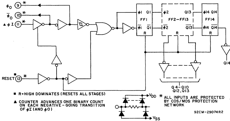
Fig. 1 - Logic diagram.
