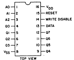
TERMINAL ASSIGNMENT
