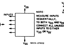
Fig. 20—Input leakage current test circuit.
