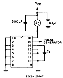
Fig. 10 - Power-dissipation test circuit.
