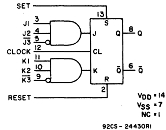
Gated J-K Master-Slave Flip-Flop, Inverting and Non-Inverting Inputs
