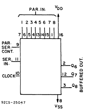
8-Stage Synchronous Shift Register with Parallel or Serial Input/Serial Output
