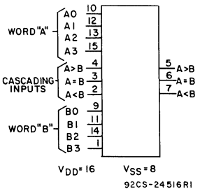
4-bit Magnitude Comparator CD4063B (Page 222)
