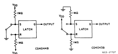
Fig. 12 – Switch bounce eliminator.
