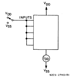
Fig. 9 – Quiescent device current.
