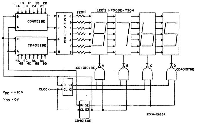
92CM-28354 Fig. 8 - Multiplexed LED circuit.
