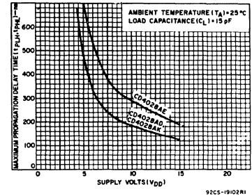
Fig. 6 - Maximum propagation delay time vs. V DD .
