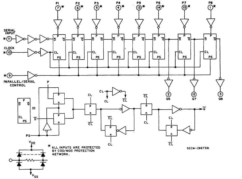
Fig. 1 - Logic diagram for CD4014B.
