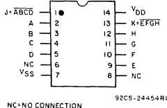
TOP VIEW CD4012UB
