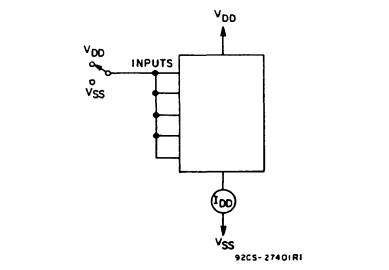
Fig. 14 - Quiescent-device-current test circuit.
