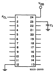
Fig. 19 - Power dissipation test circuit (all \div modes).
