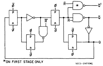
Fig. 4 — Detail of typical flip-flop stage.
