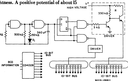
Fig. 15 - Series-type multiplexing of a one-of-ten gas-discharge display.
