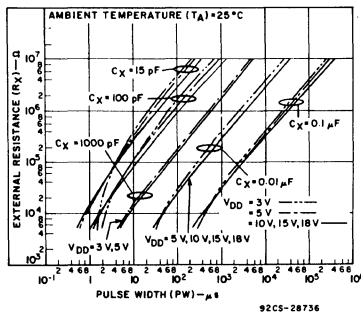
Fig. 8 - Typical external resistance vs. pulse width.
