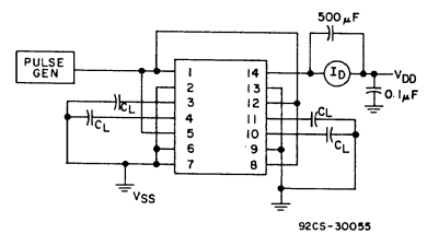
Fig. 13 - Dynamic power dissipation test circuit.
