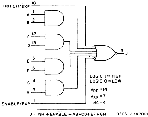
Expandable 4-Wide, 2-Input AND-OR-INVERT (AOI) Gate
