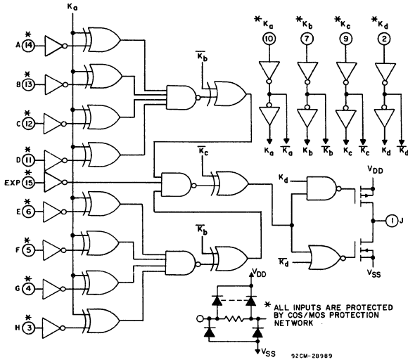
Fig. 2 — Logic diagram.
