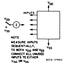
Fig. 8—Input-leakage-current test circuit.
