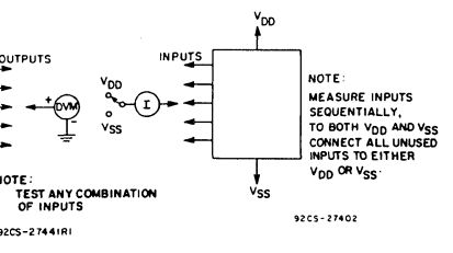
Fig. 10 — Input voltage test circuit.
