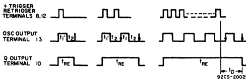
Fig. 29 - Retrigger-mode waveforms.
