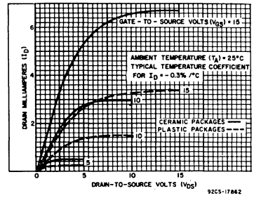
Fig. 4—Minimum output n-channel drain characteristics.
