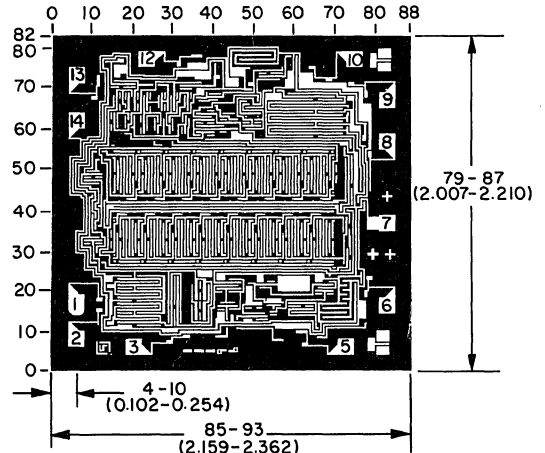
Dimensions and pad layout for CD4541B.
