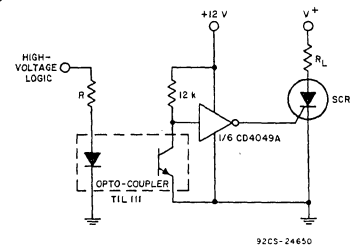
Fig. 18—High-voltage logic to COS/MOS driving an SCR.
