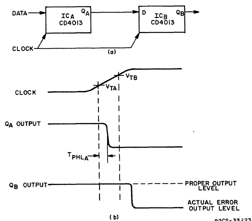
Fig.1-Parallel clocking of sequential CMOS IC's.
