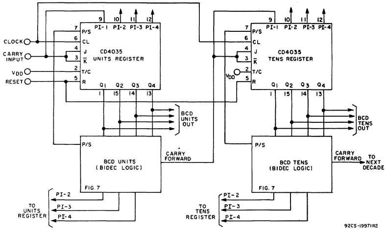
Fig. 17 - Binary-to-BCD converter.
