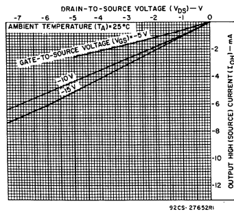
Fig. 12 — Minimum output high (source) current characteristics.
