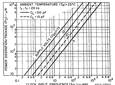
Fig.9 - Typical dynamic power dissipation vs. frequency.
