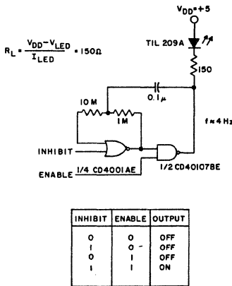
92CS-28353R1 Fig. 7 - LED driver circuit.
