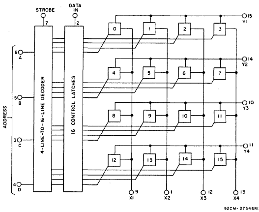
4-by-4 Crosspoint Switch with Control Memory CD22100 (Page 636)
