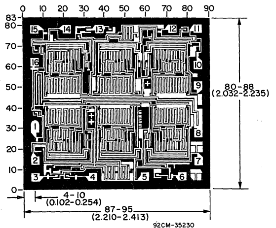
Dimensions and Pad Layout for CD4502BH
