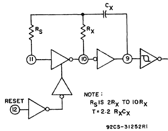
Fig. 12 — Typical RC circuit.
