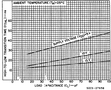
Fig. 18 - Typical high-to-low transition time vs. load capacitance.
