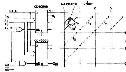
Fig. 16 - Multiple selection decoding - 4 x 4 crosspoint switch.
