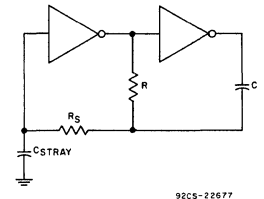
Fig. 7 — RC-oscillator circuit with stray capacitance.
