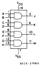
Quad 2-Input AND Gate
