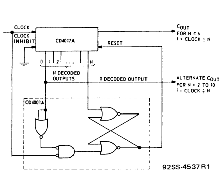
Fig. 12 - Divide by N counter ( N \leq 10 ) with N decoded outputs.
