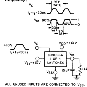
Fig. 10 - Maximum allowable control input repetition rate.
