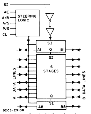
92CS-29108 8-Stage Static Bidirectional Parallel/Serial Input/Output Bus Register CD4034A (Page 549) CD4034B (Page 158)
