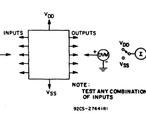
Fig. 11 — Input voltage test circuit.
