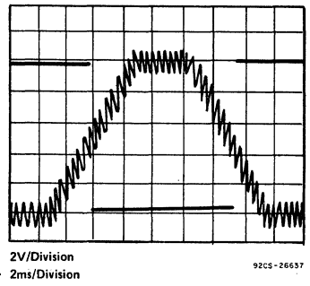
Fig.19 - Rejection of noise on slow input edge.
