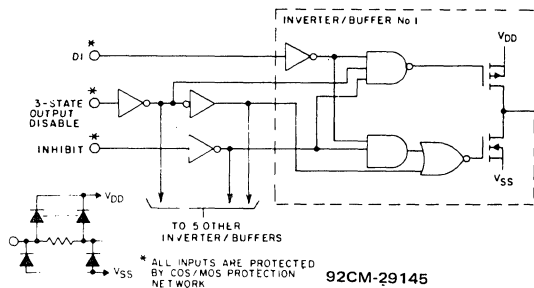
Fig.1 - Logic diagram of 1 of 6 identical inverter/buffers.
