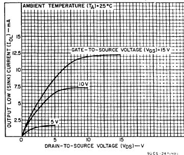
Fig.10 — Minimum output low (sink) current characteristics.
