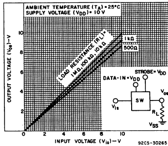
Fig. 7 - Typical switch ON transfer characteristics (1 of 16 switches).
