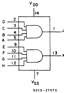
Dual 4-Input AND Gate
