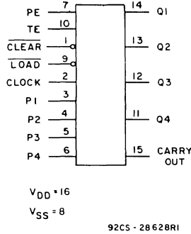
Synchronous 4-Bit Counter
