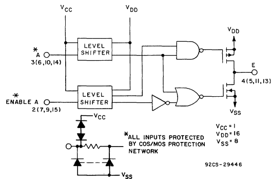
Fig. 1 - CD40109B logic diagram (1 of 4 units).
