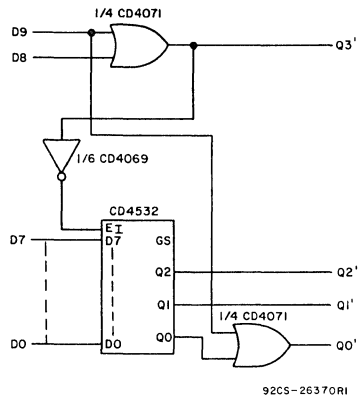
Fig. 15 - 16-level priority encoder.
