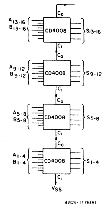
Fig. 10 - Typical connection for a 16-bit adder.
