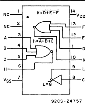
Dual 3-Input NOR Gate Plus Inverter
