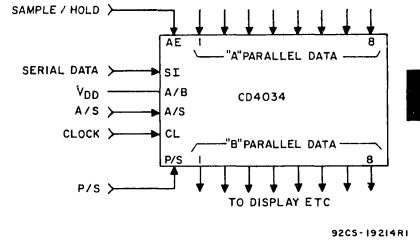
Fig. 22 - Sample and hold register-serial/parallel in-parallel out.
