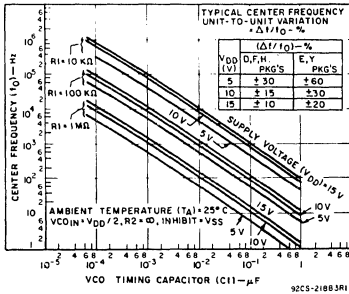
Fig.5(a) - Typical center frequency vs C_1 for R_1 = 10\text{ k}\Omega , and 1\text{ M}\Omega and f_0 \approx 1/R_1 C_1 .
