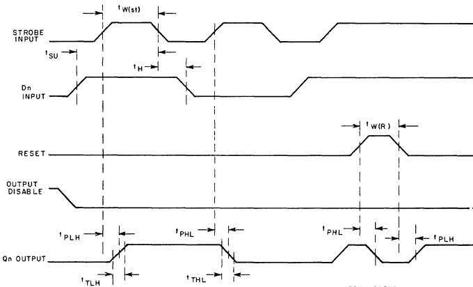
Fig.12 - Test waveforms.
