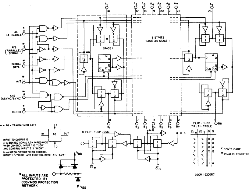
Fig. 2 — Logic diagram.
