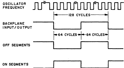
Fig. 6 - Display waveforms.
