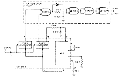
Fig. 15— Lock-detection circuit.
