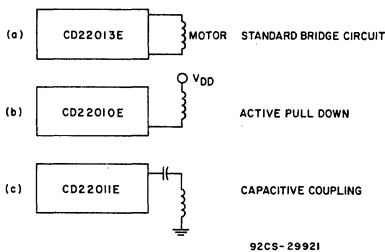
Fig. 5 - Typical motor interface circuits for analog watch or wall clock circuits.
