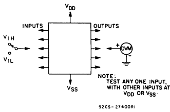
Fig. 21 - Noise immunity test circuit.
