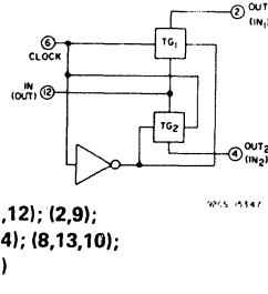
h) Dual Bi-Directional Transmission Gating
