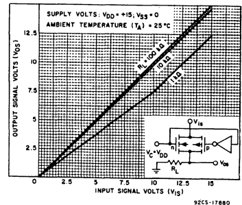
Fig. 2—Typ. "ON" characteristics for 1 of 4 switches with V_{DD} = +15 \text{ V} , V_{SS} = 0 \text{ V} .
