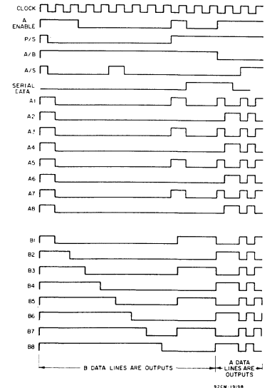
Fig. 4 — Timing diagram.
