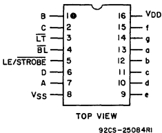
CD4511B TERMINAL ASSIGNMENT
