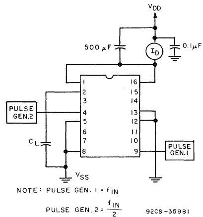
Fig. 10 - Dynamic power dissipation test circuit.
