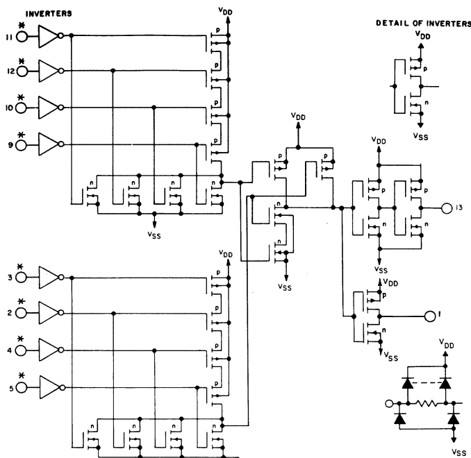
Fig. 7 - Schematic diagram.
