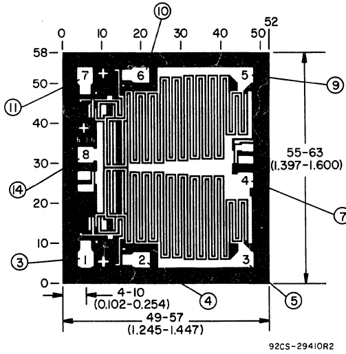
Dimensions and Pad Layout for CD40107BH.
