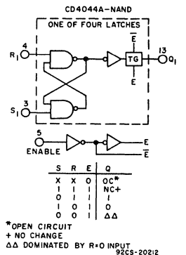
Fig. 1 - Logic diagrams and truth tables.
