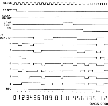
Fig. 4 - CD4033B timing diagram.
