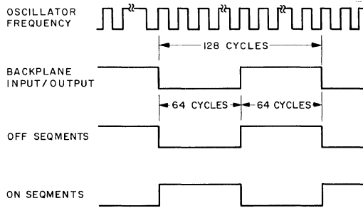
Fig. 6 - Display waveforms.
