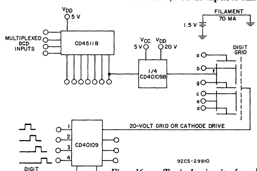
Fig. 16 - Typical circuit for driving a fluorescent digital display.
