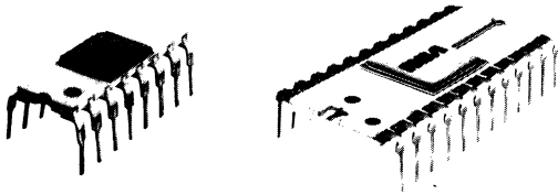
18, 22, 24, 40-Lead Side-Brazed Versions
