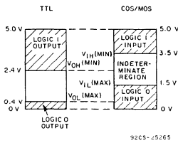
Fig. 1—TTL to COS/MOS voltage levels.
