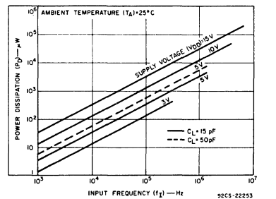
Fig. 6— Typical power dissipation as a function of input frequency.
