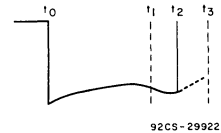
Fig. 4 - Nominal output pulse of stepper motor.
