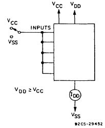
Fig. 13 - Quiescent device current.
