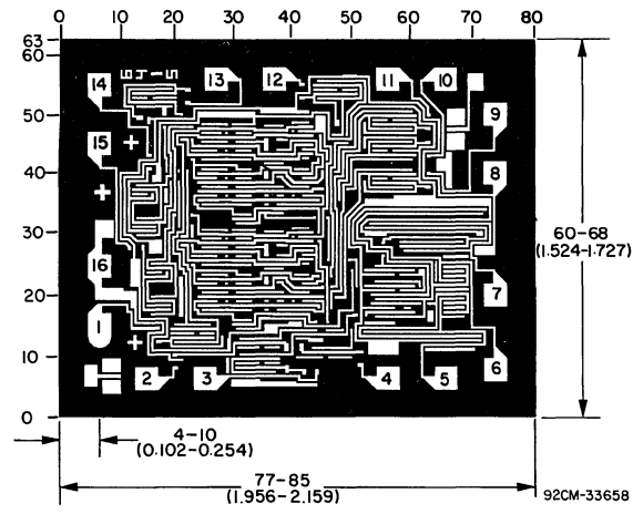
Dimensions and pad layout for CD4063BH.
