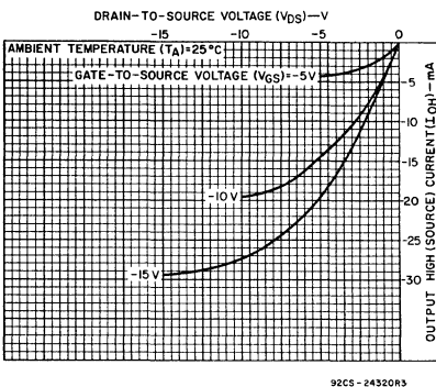
Fig. 5 - Typical carry or borrow output high (source) current characteristics.
