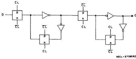
Fig. 3 - Logic diagram.
