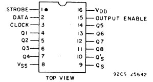
Fig. 1 — Terminal assignment.
