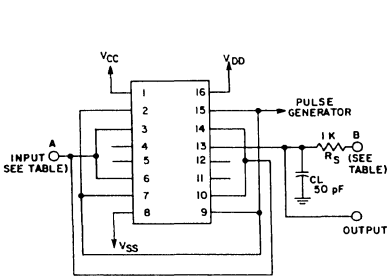
Fig. 12 - Output enable delay times test circuit and waveforms.
