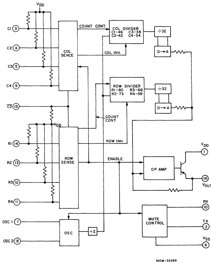
Fig. 2 - Touch-tone generator.
