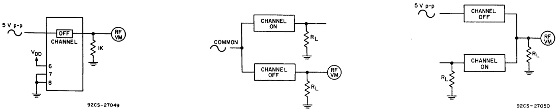
Fig. 25 - Crosstalk between any two channels (all types).
