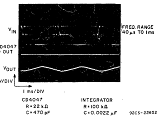
Fig. 26 - Frequency-discriminator-circuit waveforms.
