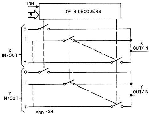
Differential 8-Channel Multiplexer/Demultiplexer CD4097B (Page 231)
