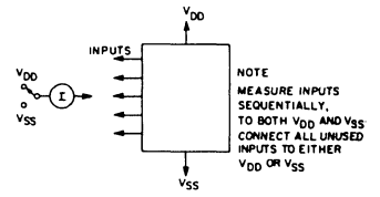
Fig. 9 — Input-leakage-current test circuit.
