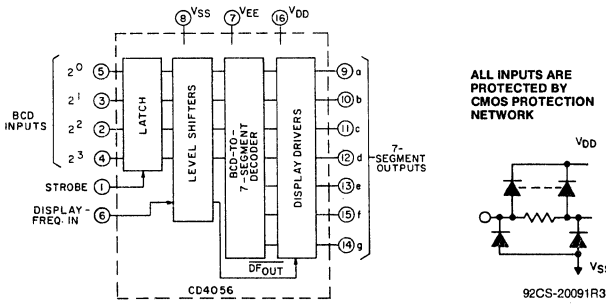
Fig.3 - CD4056B functional diagram.
