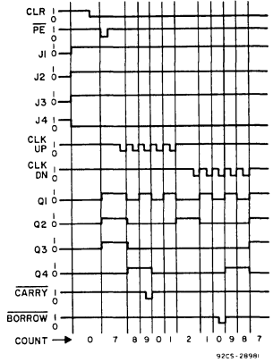
Fig. 3 — CD40192B timing diagram.
