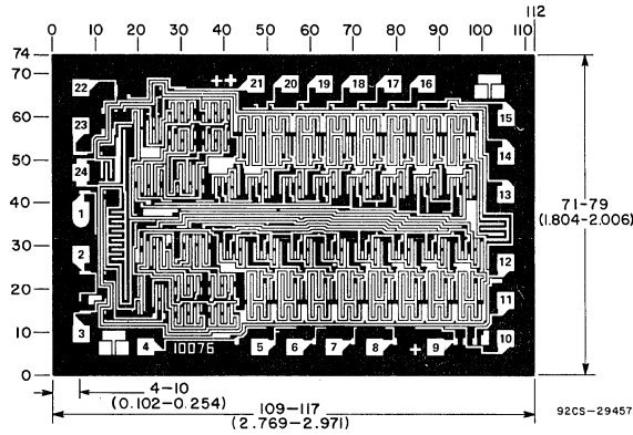
Dimensions and Pad Layout for CD4515B Chip (Dimensions and pad layout for the CD4514B are identical)
