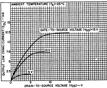
Fig. 9 — Minimum output low (sink) current characteristics.
