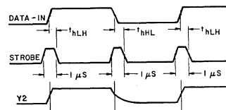
Fig. 21 - Strobe to Data-In hold time t_{HI} for CD22101.
