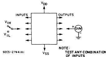
Fig.13 — Input voltage test circuit.
