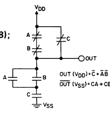
Fig. 2 - Sample COS/MOS logic circuit arrangements using type CD4007UB.
