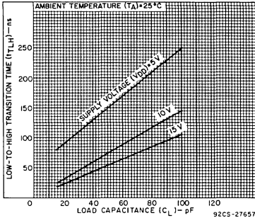
Fig. 17 - Typical low-to-high transition time vs. load capacitance.
