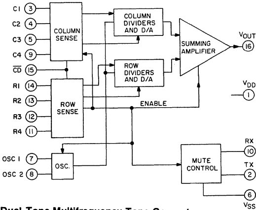
Dual-Tone Multifrequency Tone Generator
