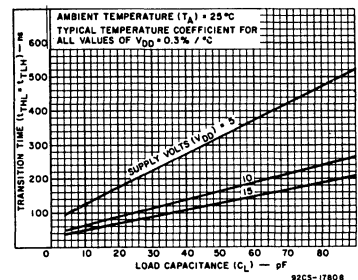
Fig. 6 - Typical transition time vs. load capacitance.
