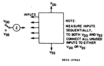
Fig. 12 - Input current test circuit.
