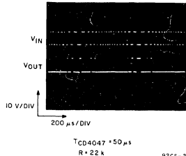
Fig. 29 - Low-pass-circuit waveforms.
