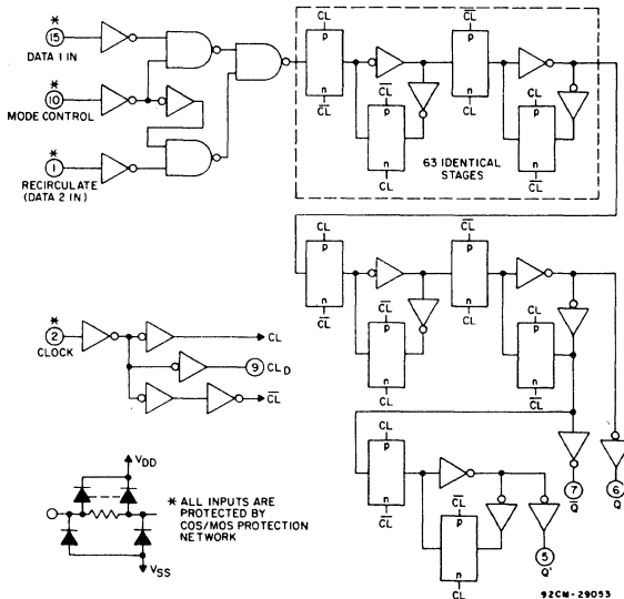
Fig. 1 - Logic diagram.
