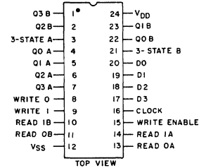
92CS-27697 TERMINAL ASSIGNMENT
