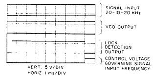
Fig. 16— Lock-detection-circuit waveforms.
