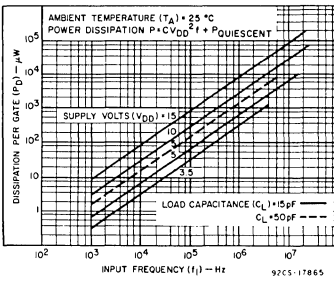
Fig. 14 — Typical power dissipation vs. frequency.
