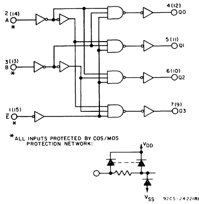
Fig. 6 - CD4555B logic diagram (1 of 2 identical circuits).
