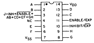
Top View TERMINAL ASSIGNMENT
