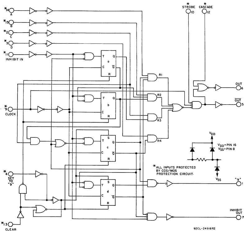
Fig. 13 — Logic diagram.
