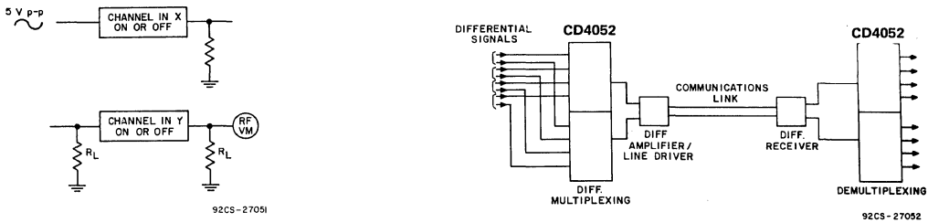
Fig. 26 - Crosstalk between duals or triplets (CD4052B, CD4053B).
