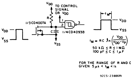
Fig. 17 — Monostable multivibrator.
