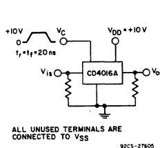
Fig.18 - Crosstalk-control input to signal output.
