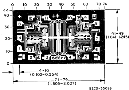
Dimensions and Pad Layout for CD4093BH
