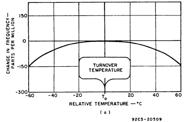
Fig. 7— Effect of temperature on crystal frequency.
