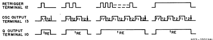
Fig. 34—Retrigger-mode waveforms.
