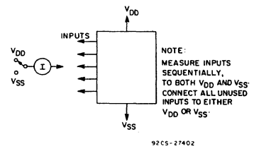
Fig. 15 – Input leakage current.
