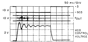
Fig. 13— Frequency-synthesizer waveforms.
