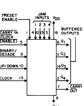
92CS-17190R3 Presettable Up/Down Counter, Binary or BCD-Decade CD4029A (Page 538) CD4029B (Page 140)
