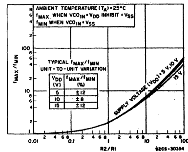
Fig. 8 — Typical f_{MAX}/f_{MIN} as a function of R2/R1 .
