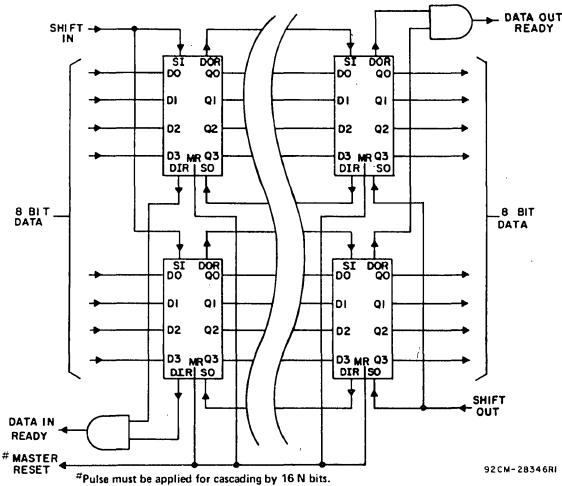
Fig. 15 - Expansion, 8-bits-wide-by-16 N-bits long using CD40105B.
