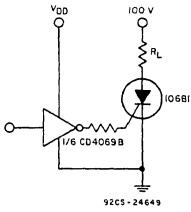
Fig. 17—COS/MOS directly driving a sensitive-gate SCR.
