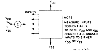
Fig. 19 — Input current test circuit.
