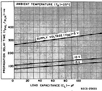
Fig. 8 — Clock-to-serial output Q_S propagation delay vs C_L .
