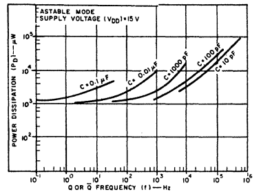
Fig. 32 - Power dissipation vs output frequency ( V_{DD} = 15 V).
