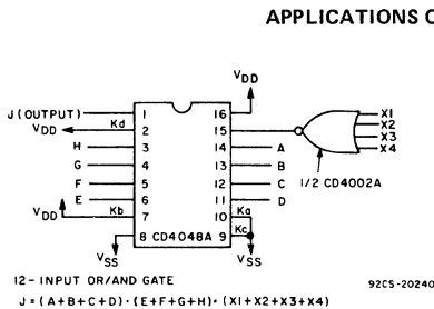
Fig. 4 — 12-input OR/AND gate.
