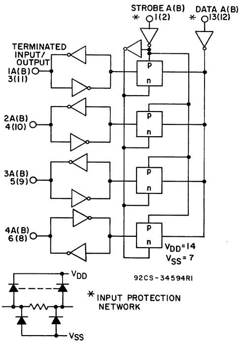
Fig. 1 - Logic diagram (1/2 CD40117B)
