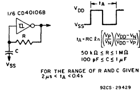
Fig. 18 - Astable multivibrator.
