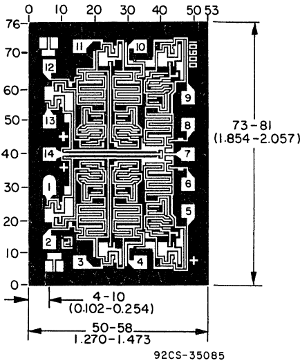
Dimensions and Pad Layout for CD40106BH
