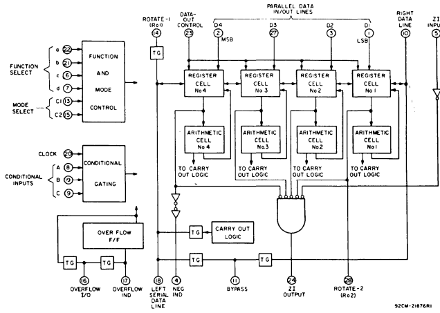
4-bit Arithmetic Logic Unit CD4057A (page 593)
