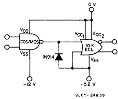
Fig. 8—COS/MOS at 12 volts to 10k-ECL interface.
