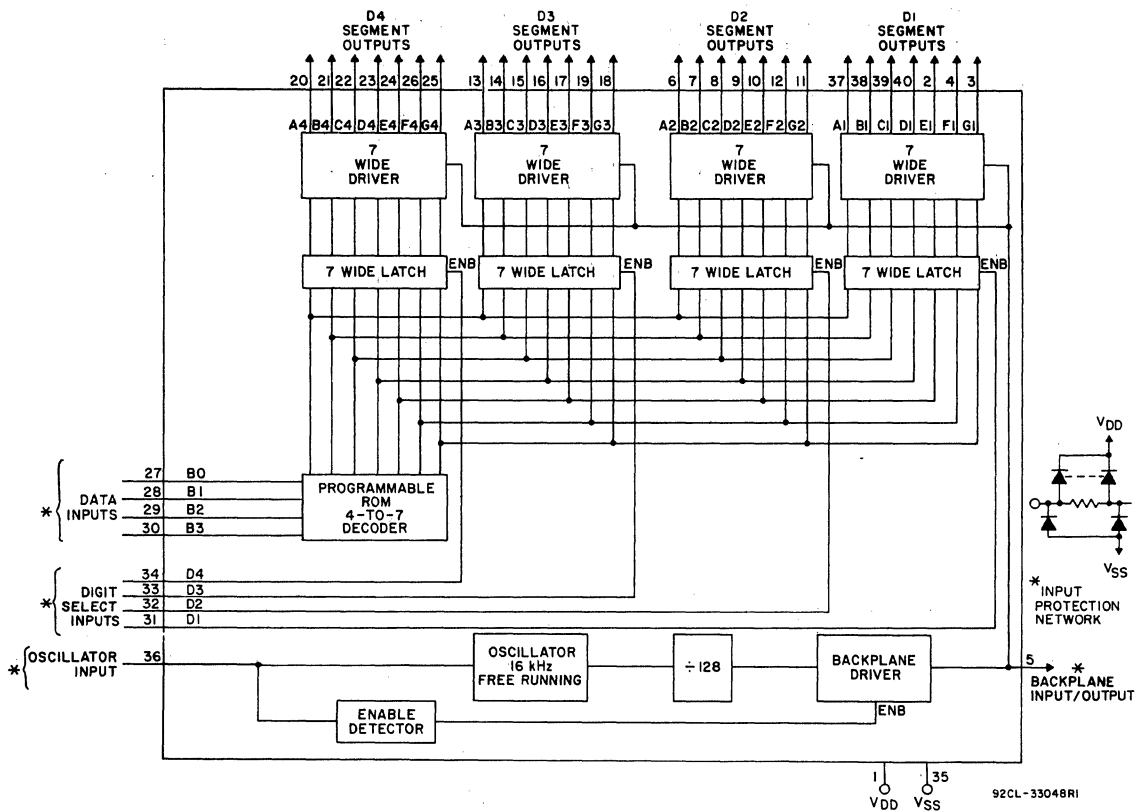
Fig. 1 - Block diagram of CD22104 and CD22104A.
