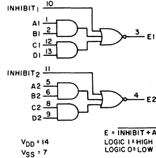
Dual 2-Wide, 2-Input AND-OR-INVERT (AOI) Gate
