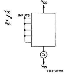
Fig.18 – Quiescent device current test circuit.
