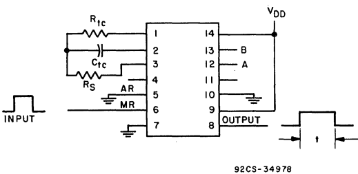
Fig. 3 - Digital timer application circuit.
