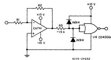
Fig. 20—Split-rail op-amp to COS/MOS interface.
