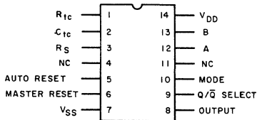
TERMINAL ASSIGNMENT
