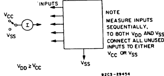
Fig. 15 - input current.
