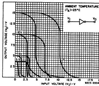
Fig. 11 — Minimum and maximum transfer characteristics — complement output.
