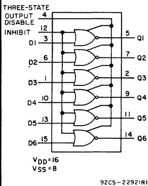
Strobed Hex Inverter/Buffer CD4502B (Page 295)
