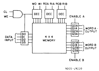
Fig. 1 - Block diagram.
