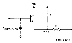
Fig. 16 - CD4047A clamping circuit.
