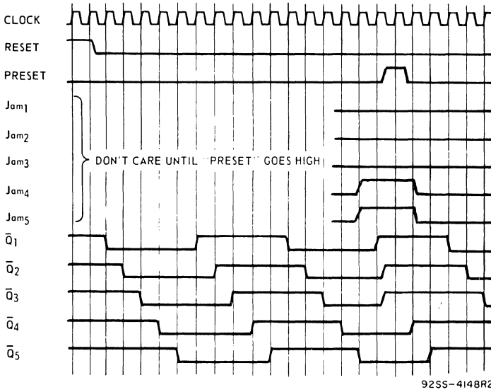
Fig. 15 — Timing diagram.
