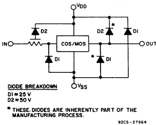
Fig. 1 — Standard protection network.
