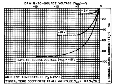
Fig. 4— Typical output p-channel drain characteristics.
