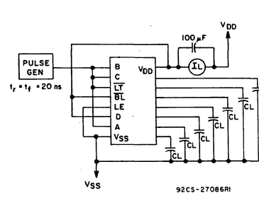
Fig. 13 - Dynamic power dissipation.
