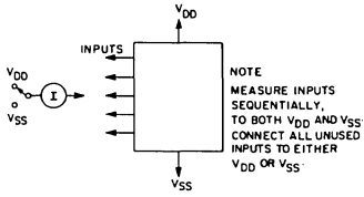
Fig. 14 - Input current test circuit.
