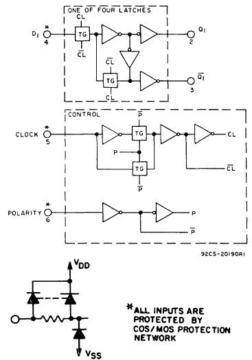
Fig. 1 - Logic block diagram & truth table.
