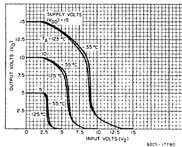
Fig. 5— Typical COS/MOS transfer characteristics as function of temperature.
