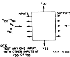
Fig. 10 - Noise immunity test circuit.
