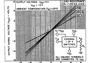
Fig. 4 - Typical ON characteristics for 1 of 4 channels.
