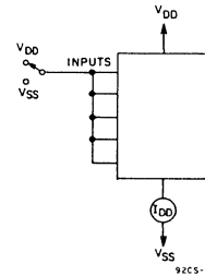
Fig. 17 — Quiescent device current test circuit.
