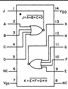
Dual 4-Input NOR Gate
