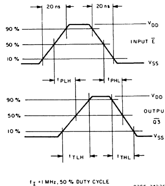
Fig. 18 - CD4556B E-bar input to Q3 output dynamic signal waveforms.
