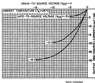
Fig. 9—Typical output high (source) current characteristics.
