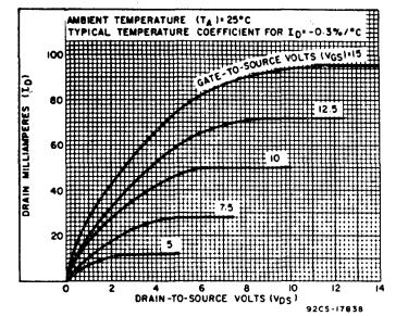
Fig. 9 - Typical n-channel drain characteristics.
