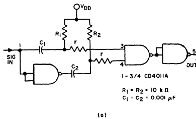
Fig. 25 - (a) Demodulator circuit, (b) waveforms.
