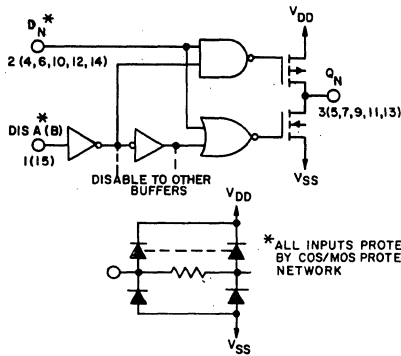
Fig. 1—Logic diagram of 1 to 6 identical buffers.
