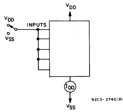
Fig. 13 — Quiescent device current test circuit.
