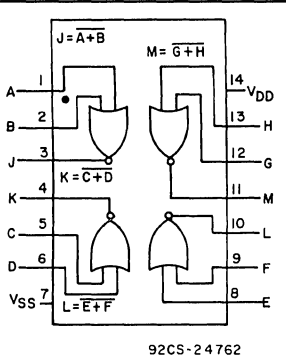
Quad 2-Input NOR Gate
