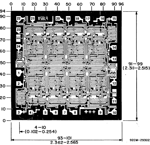
Fig. 15 — Bus register.
