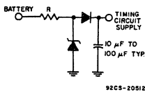
Fig. 17- Automobile transient-protection circuit.
