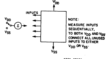
Fig.9 – Input current test circuit.
