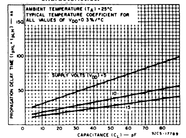
Fig. 10 — Typical propagation-delay time vs. load capacitance.
