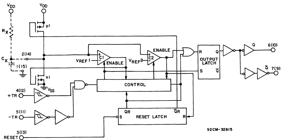
Fig. 1 - Logic diagram (1/2 of device shown).
