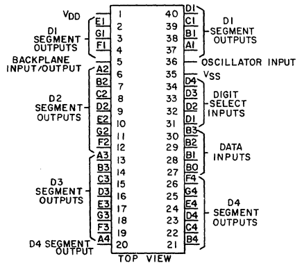
CD22104, CD22104A Terminal Assignment
