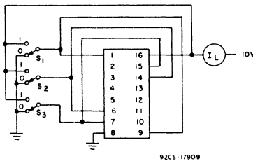
Fig. 9 — Quiescent-device-current test circuit.
