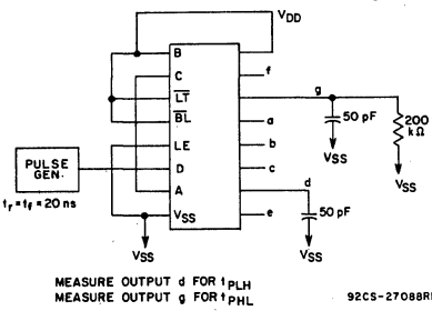
Fig. 12 - Data propagation delay.
