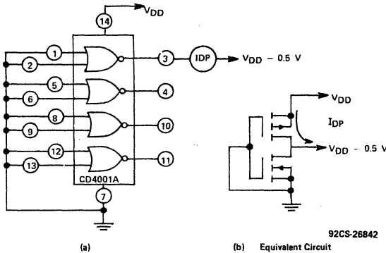
Fig. 21 - Output drive current ( I_{DP} ), source current, test arrangement.
