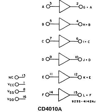
Fig. 1 — Logic diagrams.
