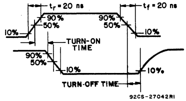
Fig. 14 - Waveforms, channel being turned ON ( R_L = 1\text{ k}\Omega ).
