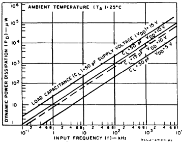
Fig. 11 - Typical dynamic power dissipation vs. frequency.
