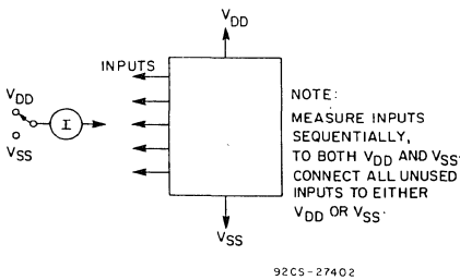
Fig. 13 - Input current.
