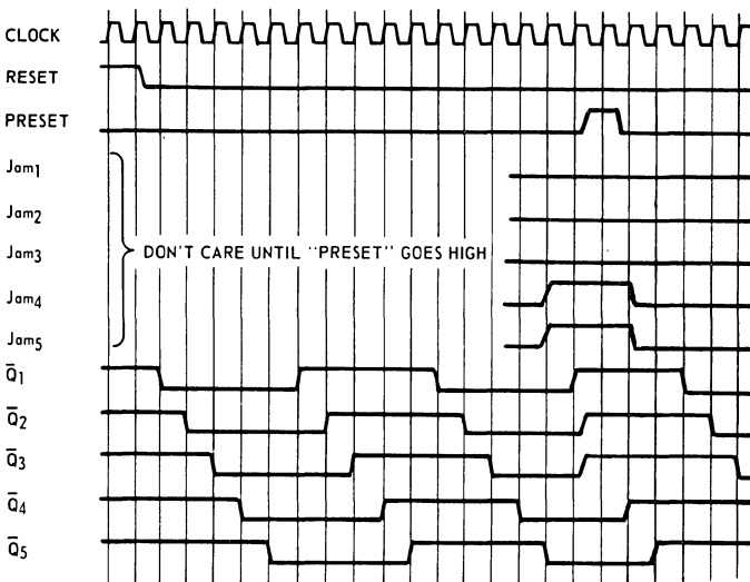
Fig. 2 - Timing diagram.
