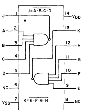
Dual 4-Input NAND Gate
