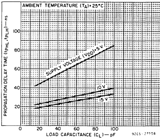
Fig. 13 — Typical propagation delay time vs. load capacitance.
