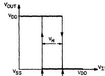
Fig. 2 - Transfer characteristic of the CD4093B.
