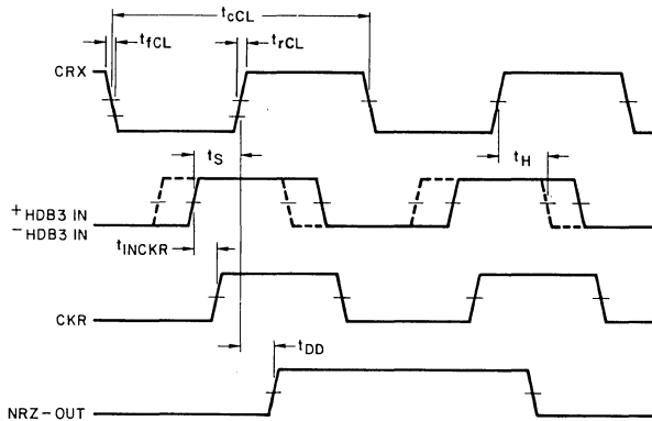
Fig. 5 - Receiver decoder timing waveforms.
