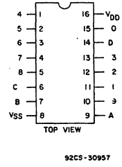
CD40147B TERMINAL ASSIGNMENT
