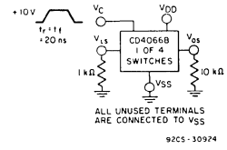
Fig. 13 — Crosstalk-control input to signal output.
