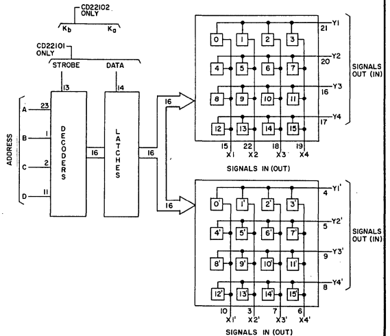
4-by-4-by-2 Crosspoint Switch with Control Memory CD22101 (Page 641) CD22102 (Page 641)
