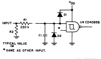
Fig.20 - Industrial-environment to COS/MOS interface.
