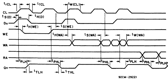
Fig. 3 - Timing diagram.
