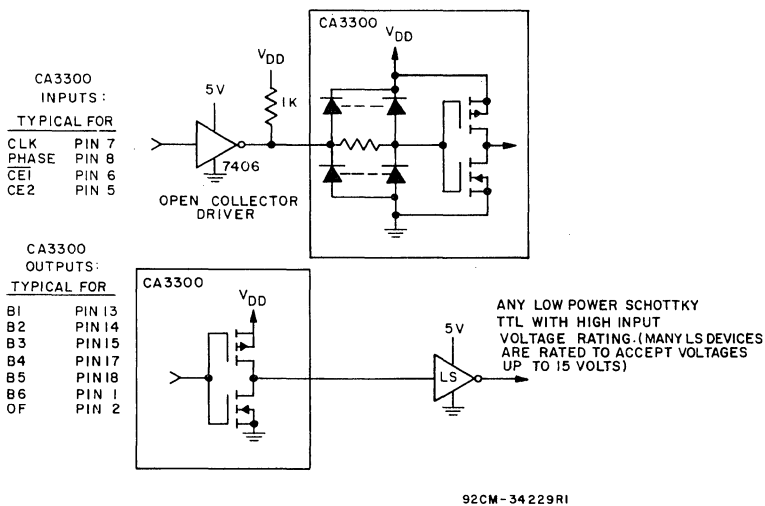
Fig. 16 - TTL interface circuit for V_{DD} > 5.5 volts.
