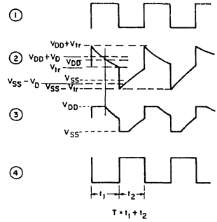
Fig. 2 - RC-oscillator operating waveforms.
