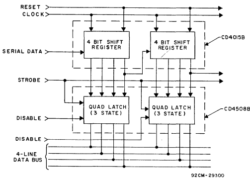
Fig. 15 — Bus register.
