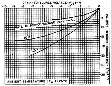
Fig. 5—Minimum p-channel output high (source) current characteristics.
