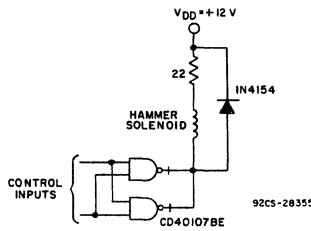
92CS-28355 Fig. 9 - Solenoid driver circuit.
