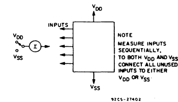
Fig. 7 - Input current test circuit.
