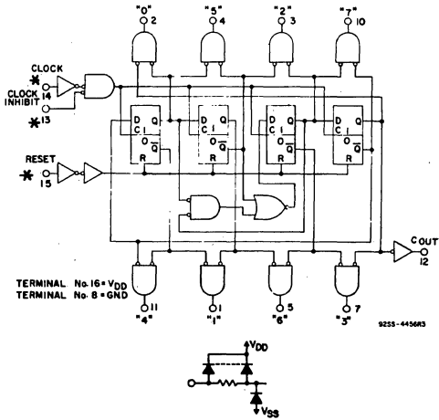
Fig. 1 — Logic diagram.
