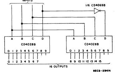
Fig. 13 – Code conversion circuit.
