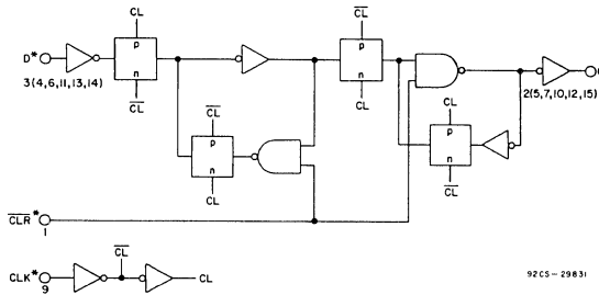
Fig. 1 - Logic diagram (1 of 6 flip-flops).
