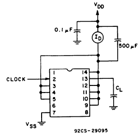
Fig. 14 - Dynamic power dissipation test circuit.
