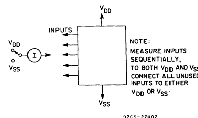
Fig. 17 - Input current.
