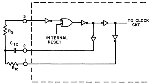
Fig. 2 — RC oscillator circuit.
