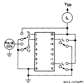
Fig. 11 - Input-leakage-current test circuit.
