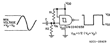
Fig.8 - Sine-wave to square-wave converter.
