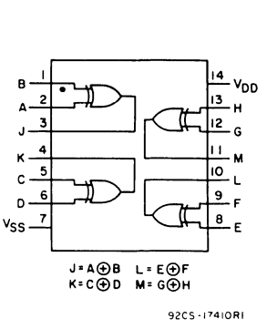
92CS-17410R1 Quad Exclusive-OR Gate CD4030A (Page 541) CD4030B (Page 146)
