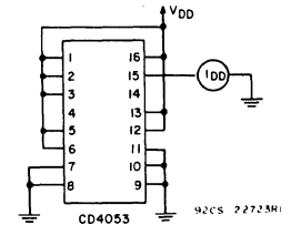
Fig. 17 - OFF channel leakage current - all channels OFF.
