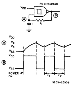
Fig.16 - Astable multivibrator.
