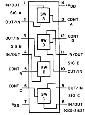
Quad Bilateral Switch CD4066A (Page 616) CD4066B (Page 226)
