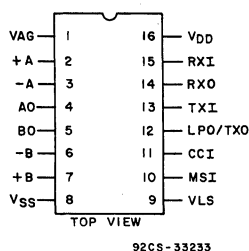
TERMINAL ASSIGNMENTS
