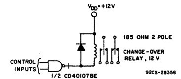
92CS-28356 Fig. 10 - Relay driver circuit.
