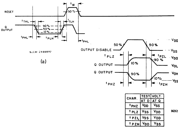
Fig. 5 — Functional waveforms for CD4076B.
