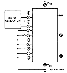
Fig. 23—Functional test circuit.
