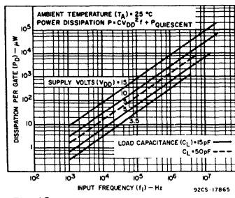
Fig. 18 — Typical dissipation characteristics.
