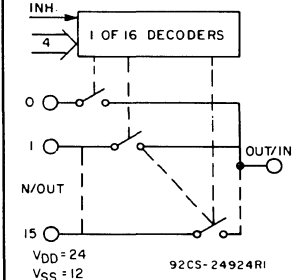
16-Channel Multiplexer/Demultiplexer CD4067B (Page 231)
