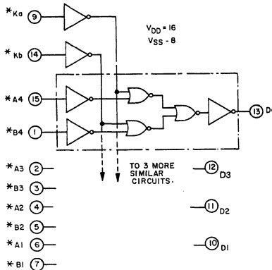
Fig. 1—Logic diagram.
