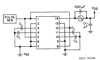
Fig. 14 – Dynamic power dissipation test circuit.
