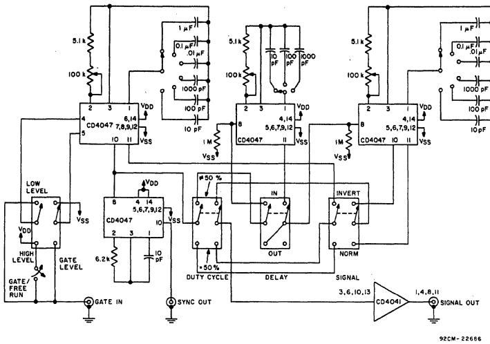
Fig. 34 - Pulse-generator circuit.
