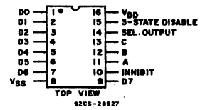
TERMINAL ASSIGNMENT
