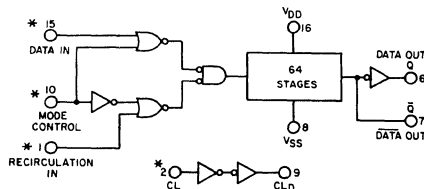
Fig. 12 - Functional diagram.
