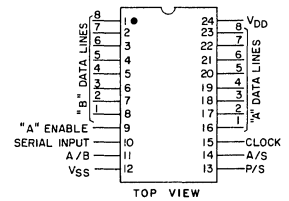
TERMINAL DIAGRAM
