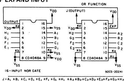
Fig. 5 — 16-input NOR gate.
