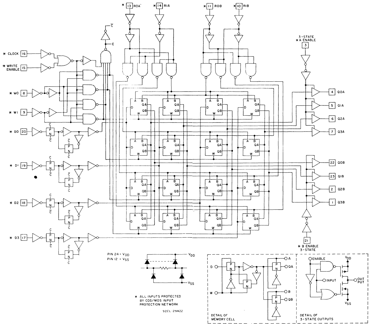
Fig. 13— Schematic diagram
