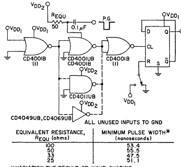
Fig. 12 Test circuit used to measure the ability of test units to withstand a negative-going noise pulse on the supply line without a change in state.
