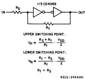
Fig. 22 — Input pulse shaping circuit (Schmitt trigger).
