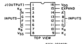
TERMINAL ASSIGNMENT
