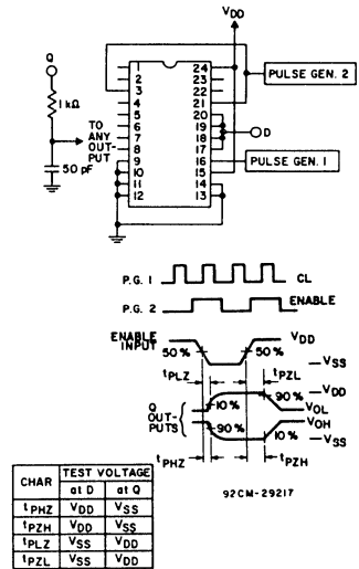
Fig. 14 — Output-enable-delay-times test circuit and waveforms.
