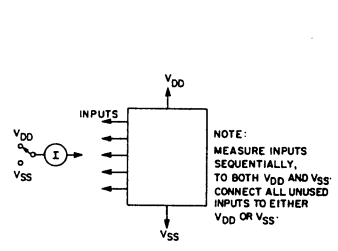
Fig. 13 — Input-leakage-current test circuit.
