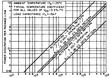
Fig. 9 - Typical power dissipation vs. frequency.
