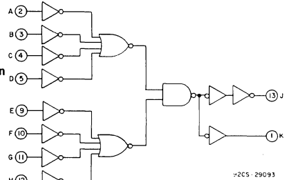
Fig. 1 - Logic diagram.
