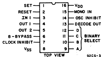
Terminal Assignment
