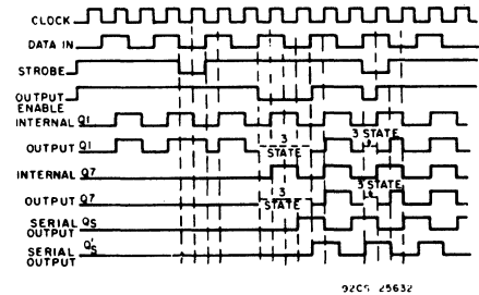
Fig. 3 — Timing diagram.
