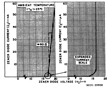
Fig. 7 - Typical zener diode characteristics.
