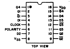
92CS-20756R1 TERMINAL ASSIGNMENT
