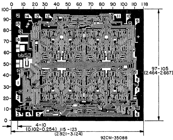
Dimensions and pad layout for CD40102B.
