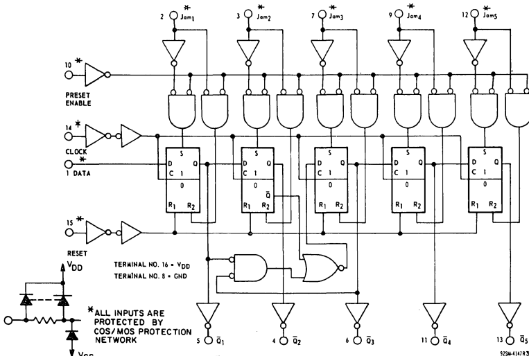
Fig. 1 - Logic diagram.
