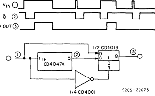
Fig. 23 - Noise-discriminator circuit.
