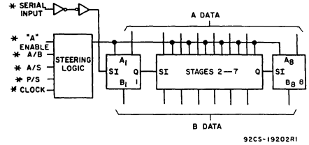
Fig. 1 - Functional diagram.
