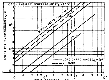
Fig. 18 — Typical dissipation characteristics.
