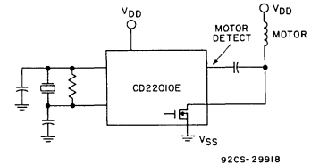
Fig. 3 - CD22010E, a low-voltage COS/MOS analog timepiece circuit, used to detect status of stepper motor current.
