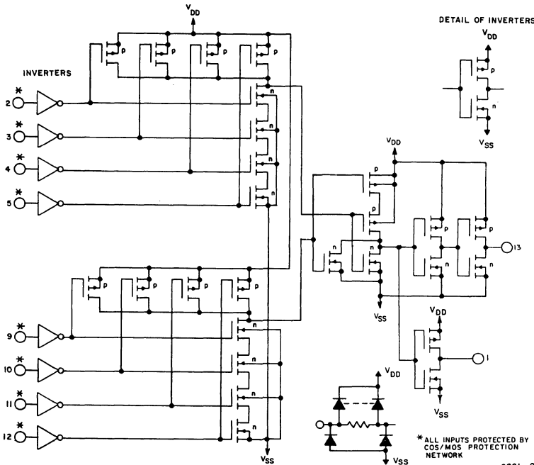
Fig. 8 - Schematic diagram.
