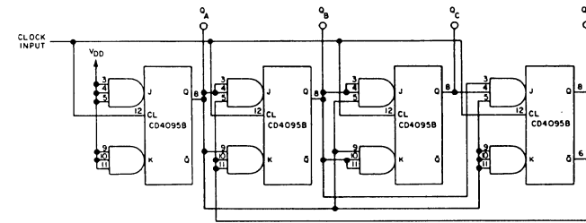
Fig. 16 - CD4095B connected in toggle mode.
