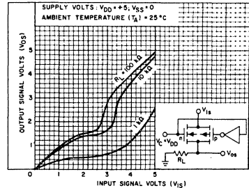
Fig. 4 - Typ. "ON" characteristics for 1 of 4 switches with V DD = +5 V, V SS = 0 V.
