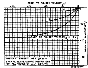
Fig. 6— Typical p-channel drain characteristics for Q output.
