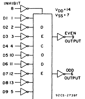
9-Bit Parity Generator/Checker
