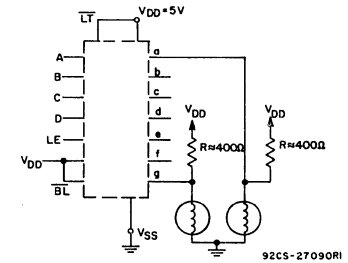
Fig. 17 — Driving incandescent displays (RCA Numitron DR2000 series displays).
