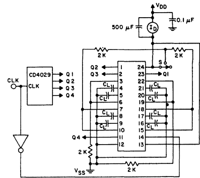
Fig. 14 - Dynamic power dissipation test circuit for CD22101.
