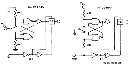
Fig. 13 - Switch bounce eliminator.
