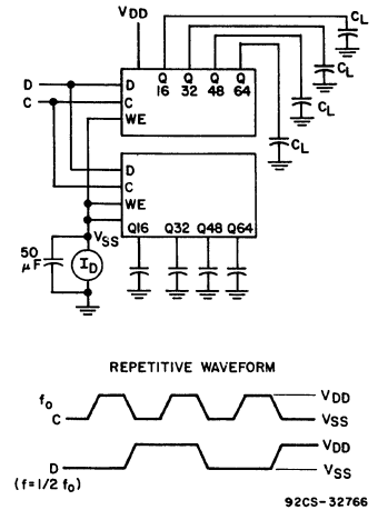
Fig. 11—Dynamic power dissipation test circuit and waveforms.
