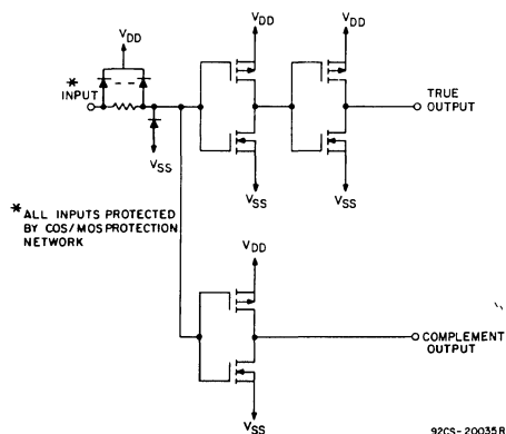
Fig. 1 — CD401A schematic diagram.
