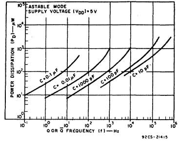
Fig. 30 - Power dissipation vs output frequency ( V_{DD} = 5 V).
