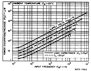
Fig. 10 — Typical dissipation characteristics.
