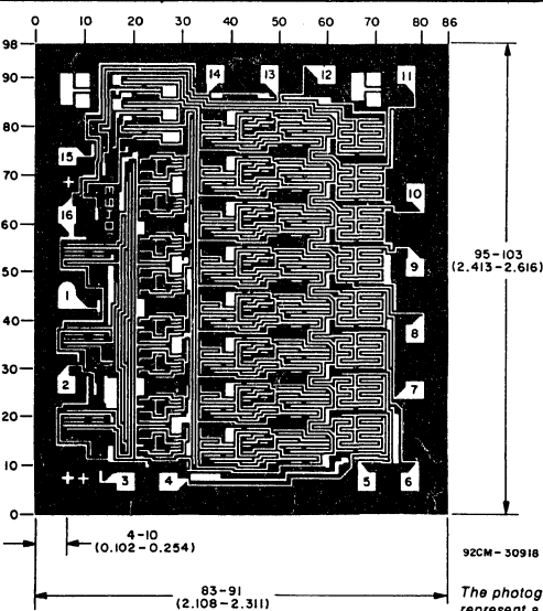
CD4724BH DIMENSIONS AND PAD LAYOUT
