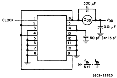
Fig. 17 - Dynamic power dissipation test circuit ( \frac{1}{2} mode).
