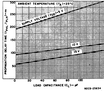
Fig. 9 — Clock-to-serial output Q'_S propagation delay vs C_L .
