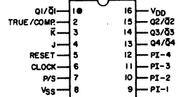
TERMINAL DIAGRAM Top View
