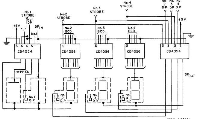
Fig. 19 — Typical 3 1/2-digit liquid-crystal display: V_{DD} = +5\text{ V} , V_{SS} = 0\text{ V} , V_{EE} = -10\text{ V} , DF_{IN} = 30\text{ Hz} square wave.
