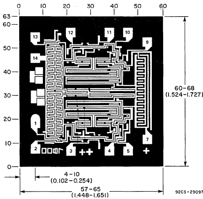
Dimensions and pad layout for CD4068BH.
