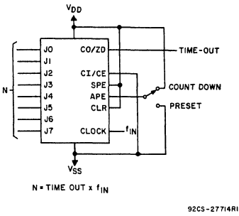
Fig. 19 - Programmable timer.
