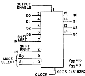
4-Bit Universal Bidirectional Shift Register 3-State Outputs
