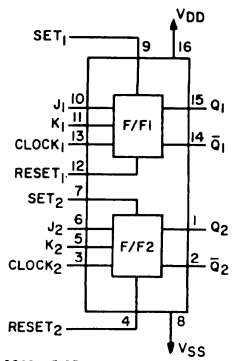
92CS-17187R1 Dual J-K Master-Slave Flip-Flop with Set-Reset Capability CD4027A (Page 532) CD4027B (Page 132)
