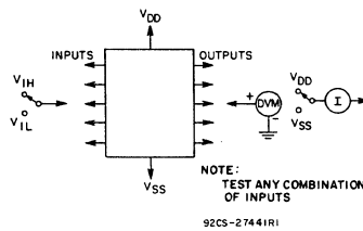
Fig. 15 – Input voltage test circuit.
