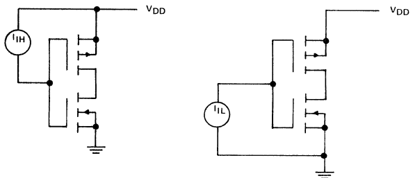
Fig. 8 — Measurement of quiescent leakage current.
