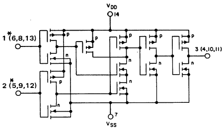
Fig. 3 - Schematic diagram for CD4071B (1 of 4 identical gates).
