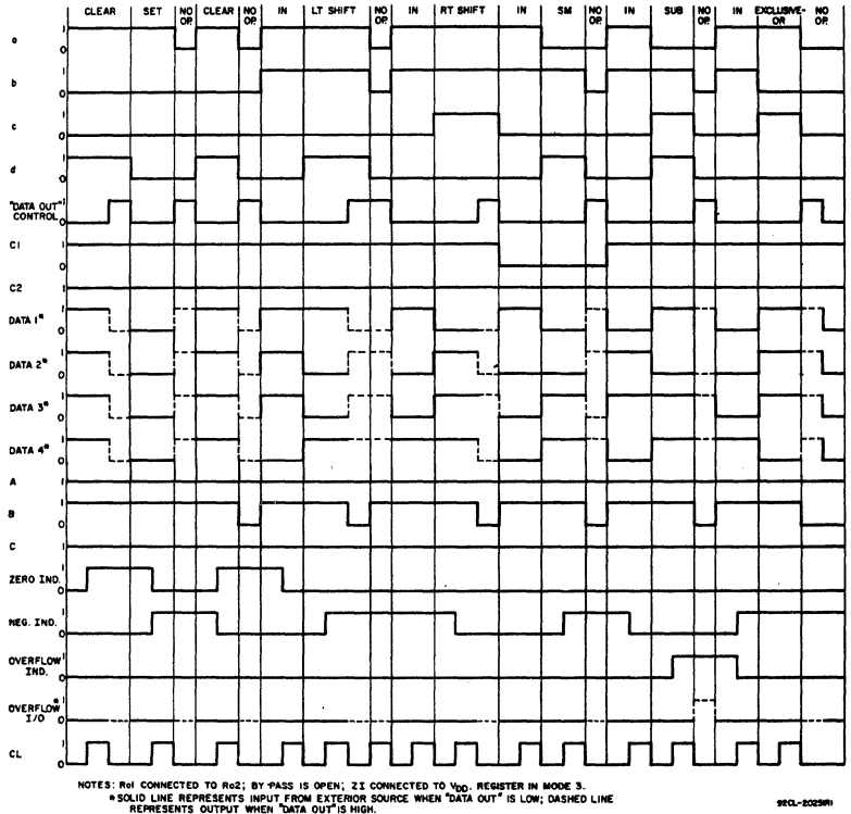
Fig. 12 – Timing diagram.
