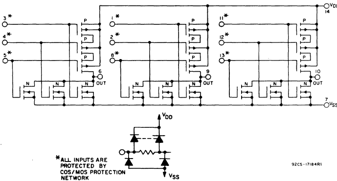
Fig. 8 - Schematic diagram for type CD4025UB.
