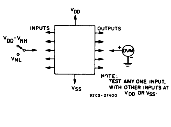
Fig. 12 — Noise-immunity test circuit.
