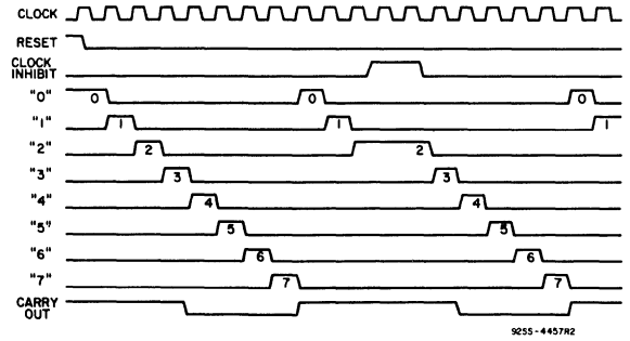
Fig. 2 — Timing diagram.
