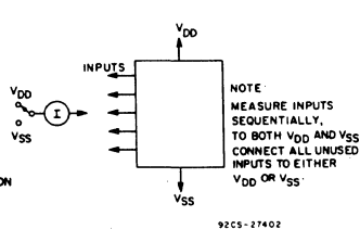
Fig. 11 – Input current.
