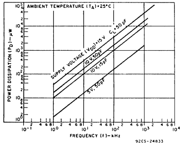
Fig. 14 — Typical power dissipation vs. frequency characteristics.
