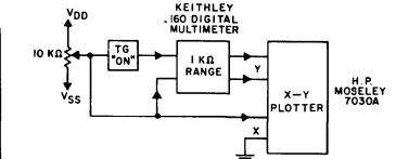
Fig. 7 - Channel on-state resistance measurement circuit.
