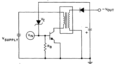
(c) Transformer-type circuit with external drive.
