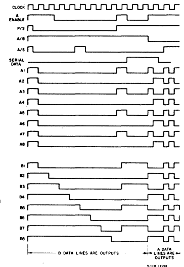
Fig. 3 — Timing diagram.
