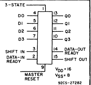
FIFO Register 4-Bits Wide by 16-Bits Long
