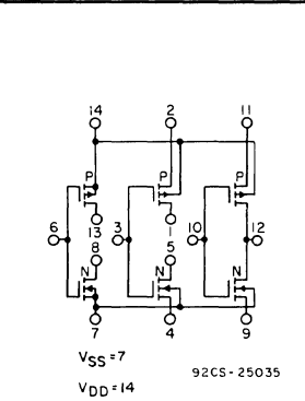
Dual Complementary Pair Plus Inverter
