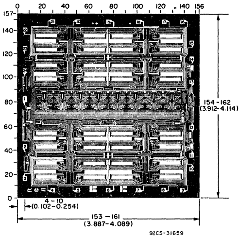
Dimensions and pad layout for CD22101H.
