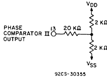
Fig. 11 — Phase comparator II output loading circuit.
