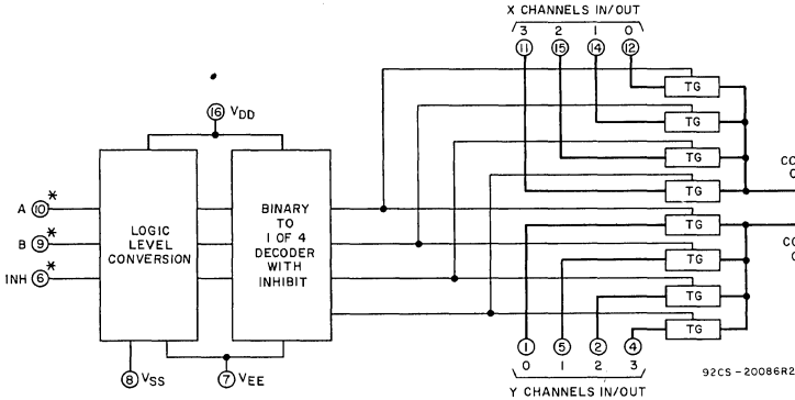
Fig. 2 - Functional diagram of CD4052B.
