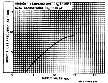
Fig. 11 — Typical input pulse frequency vs. V_{DD} .
