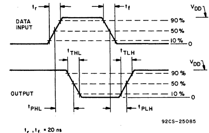
Fig. 14 - Dynamic waveforms.
