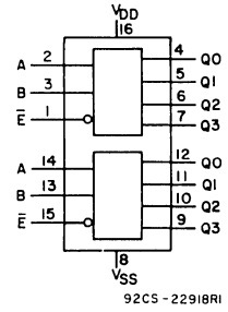
Dual Binary-to-1-of-4 Decoder/Demultiplexer Output "High" on Select CD4555B (Page 366)
