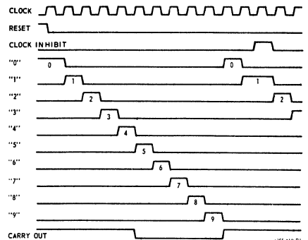
Fig. 2 - Timing diagram.
