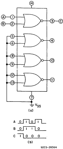
Fig. 3 - Example of CD4001 NOR-gate functional test.
