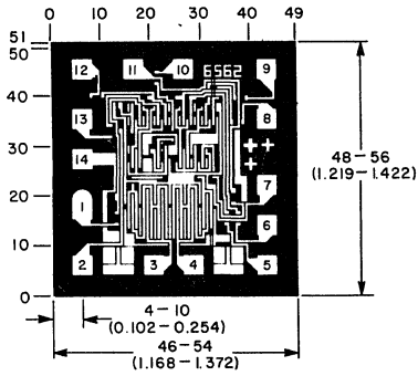
Dimensions and Pad Layout for CD4085BH.
