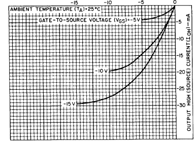
Fig. 7 - Typical output high (source) current characteristics.
