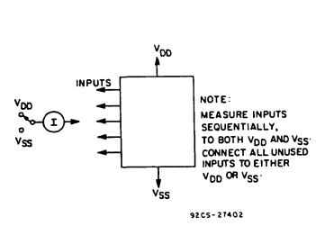
Fig. 11 - Input current test circuit.
