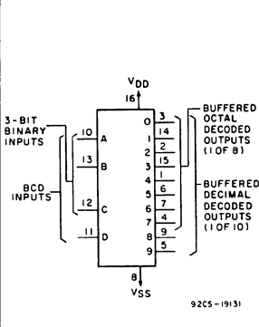
92CS-19131 BCD-to-Decimal Decoder CD4028A (Page 535) CD4028B (Page 136)
