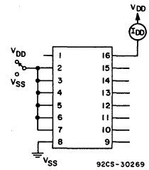
Fig. 11 - Quiescent current test circuit.
