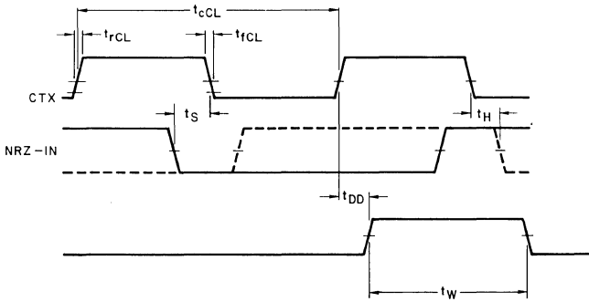
Fig. 4 - Transmitter coder timing waveforms.
