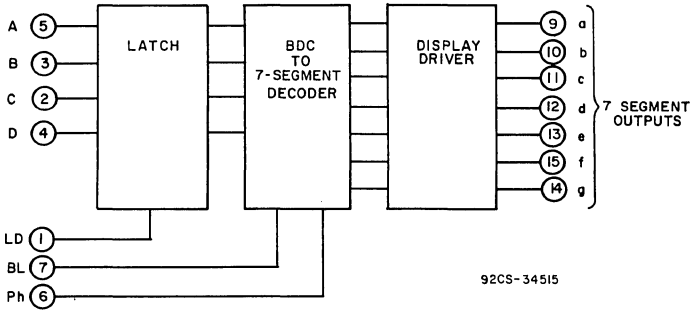
BCD-to-7-Segment Latch/Decoder/Driver CD4543B (Page 360)
