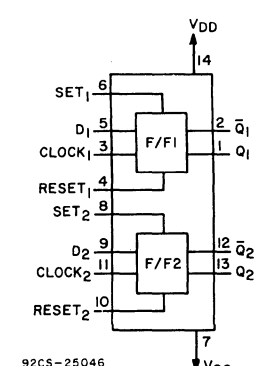
Dual 'D' Flip-Flop with Set/Reset Capability
