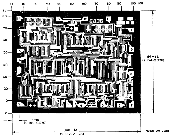
Dimensions and pad layout for CD4029B.
