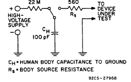
Fig. 5 — Equivalent-body discharge network.
