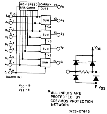
Fig. 1 — CD4008B logic diagram.
