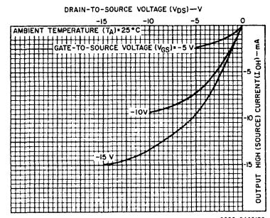
Fig. 6 - Minimum p-channel output high (source) current characteristics.
