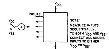
Fig. 8 - Input current test circuit.
