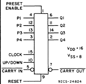
BCD Presettable Up/Down Counter CD4510B (Page 305)
