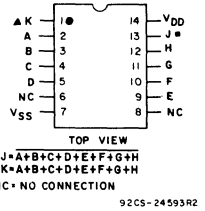
TERMINAL ASSIGNMENT
