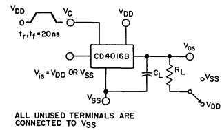
Fig. 22 - Max. control-input repetition rate.
