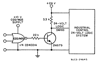
Fig. 14—COS/MOS to industrial-control interface.
