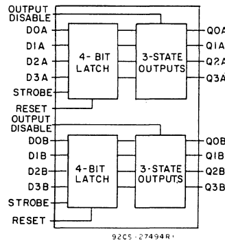
Dual 4-Bit Latch CD4508B (Page 301)
