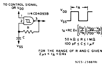
Fig. 18 — Astable multivibrator.
