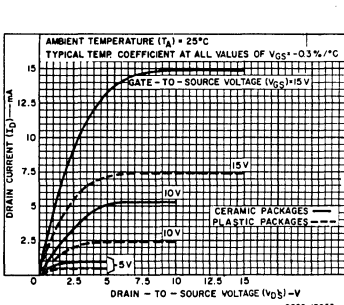
Fig. 6 - Minimum n-channel drain characteristics.
