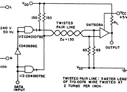
Fig. 14 - Line-driver circuit.
