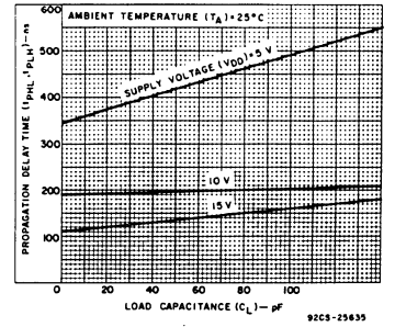
Fig. 10 — Clock-to-parallel output propagation delay vs C_L .
