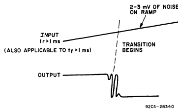
Fig. 9 — Buffered output oscillation for a slow input.
