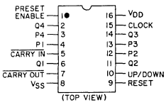
92CS-27015 CD4510B, CD4516B TERMINAL ASSIGNMENT
