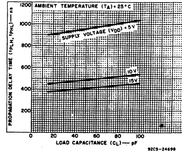
Fig. 5 - Typical propagation delay time vs. load capacitance ( \phi_4 to Q4 output).
