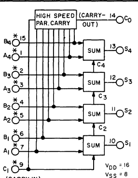
4-Bit Full Adder with Parallel Carry Out
