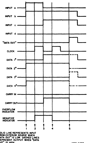
Fig. 13 – Add cycle waveforms.
