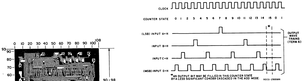
Fig. 15 - Timing diagram.
