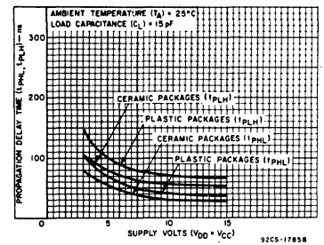
Fig. 8 - Maximum propagation delay time vs. VDD - CD4010A.
