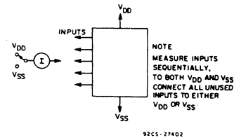
Fig. 12 - Input current.
